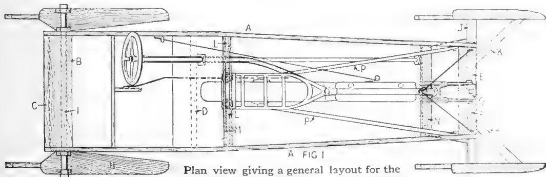
Plan view giving a general layout for the parts, frame and steering arrangement
